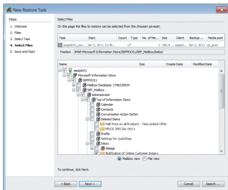
SEP sesam: Microsoft Exchange single email restore
